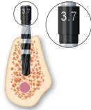
SOFT BONE SBD-3.7L 2.7/3.1 mmD Drill
